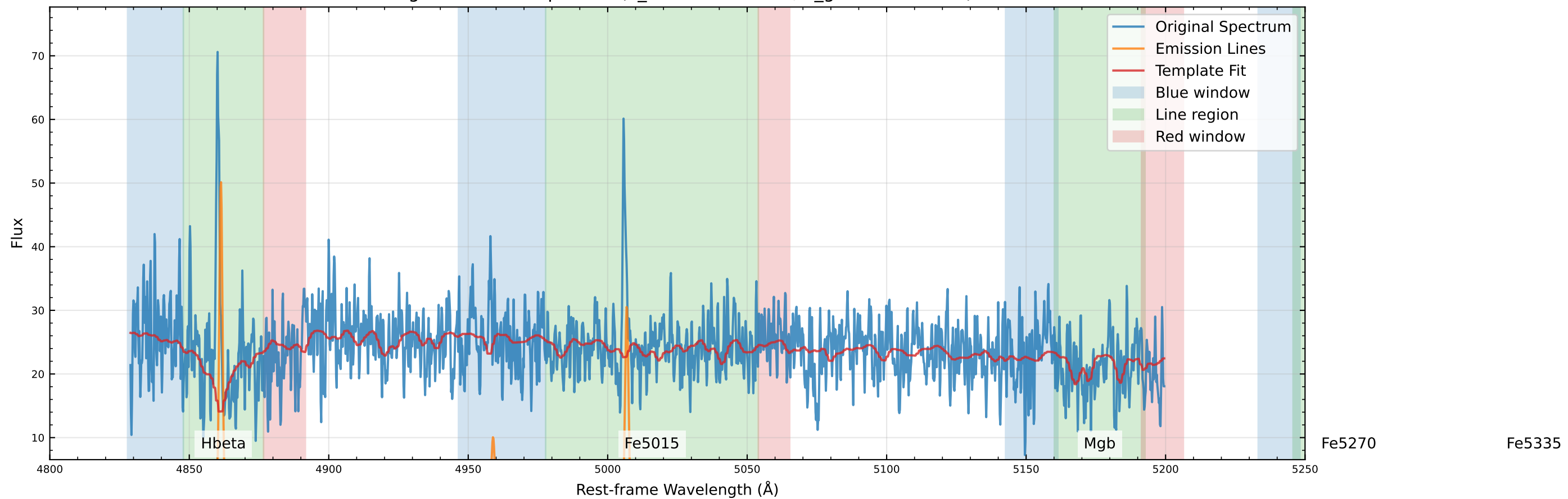
Original Data Comparison (v_star=-22.0 km/s, v_gas=-63.7 km/s)
