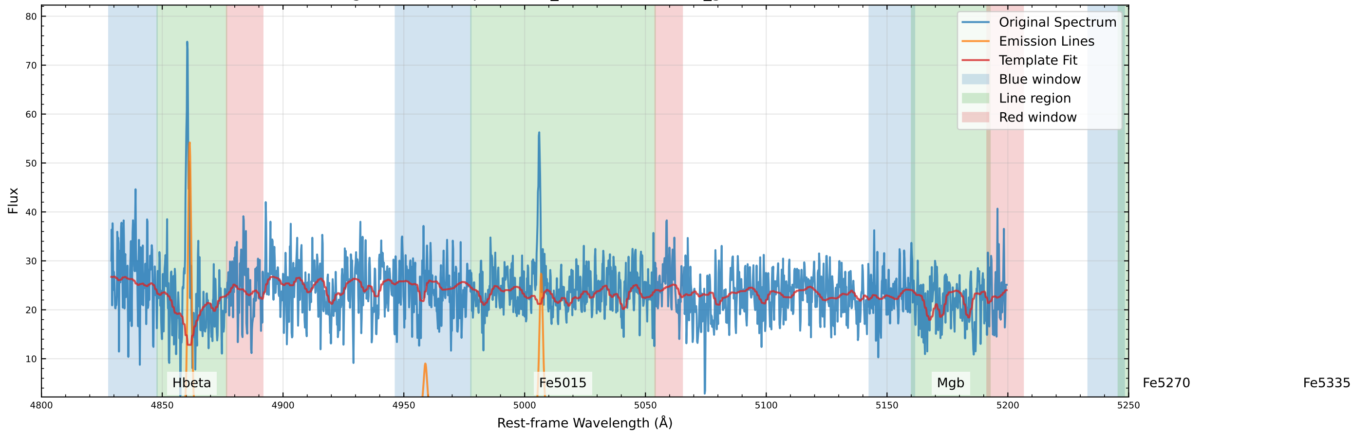
Original Data Comparison (v_star=-46.9 km/s, v_gas=-56.9 km/s)
