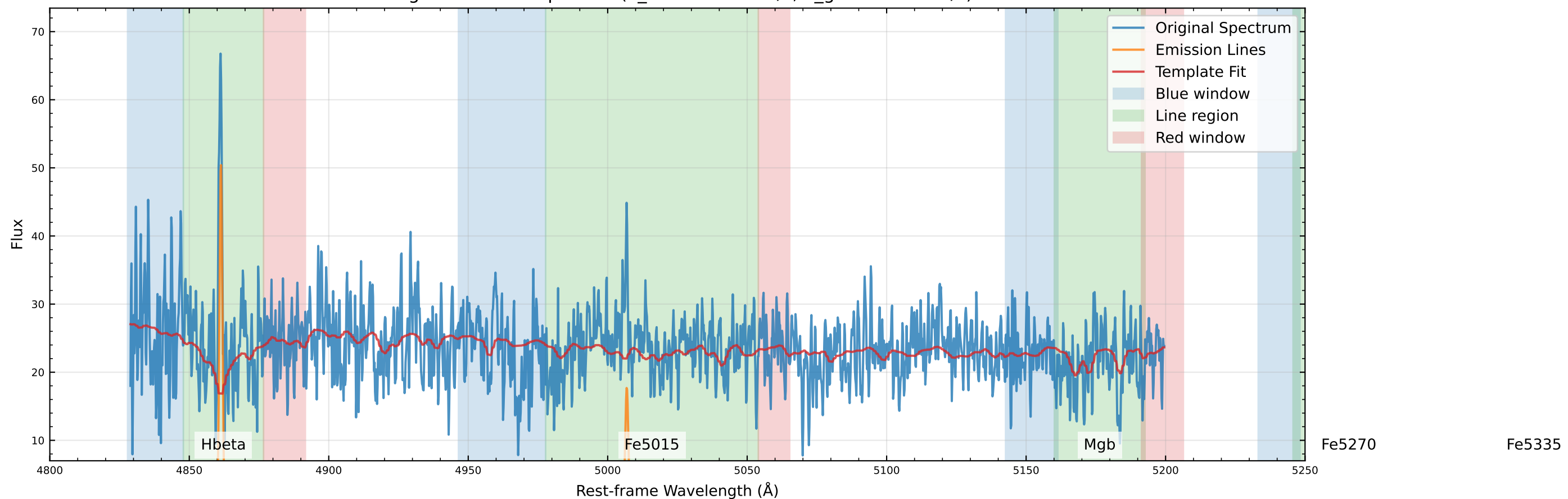
Original Data Comparison (v_star=-35.9 km/s, v_gas=-11.7 km/s)
