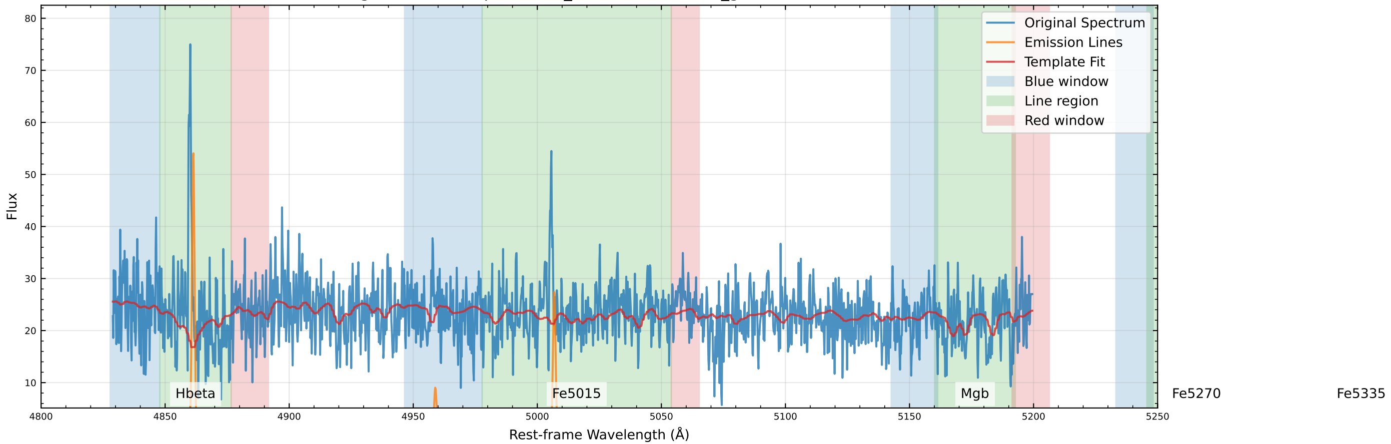
Original Data Comparison (v_star=-80.6 km/s, v_gas=-79.0 km/s)
