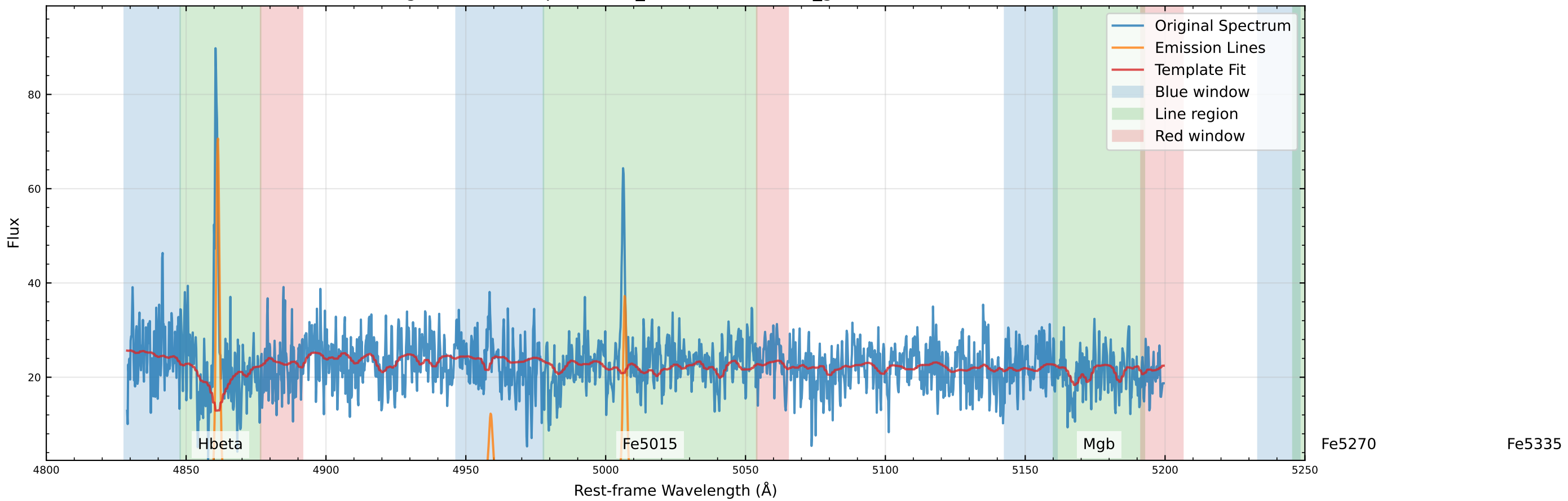
Original Data Comparison (v_star=-53.9 km/s, v_gas=-36.3 km/s)
