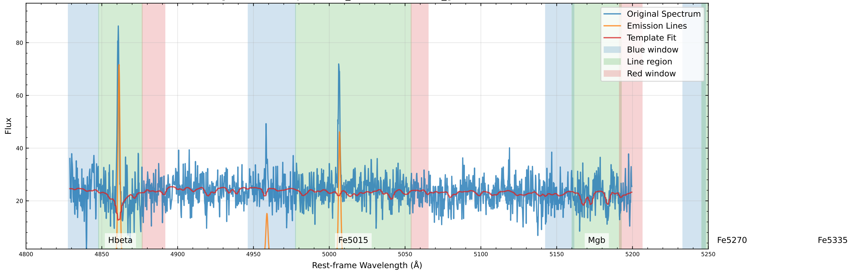
Original Data Comparison (v_star=-15.8 km/s, v_gas=-29.2 km/s)
