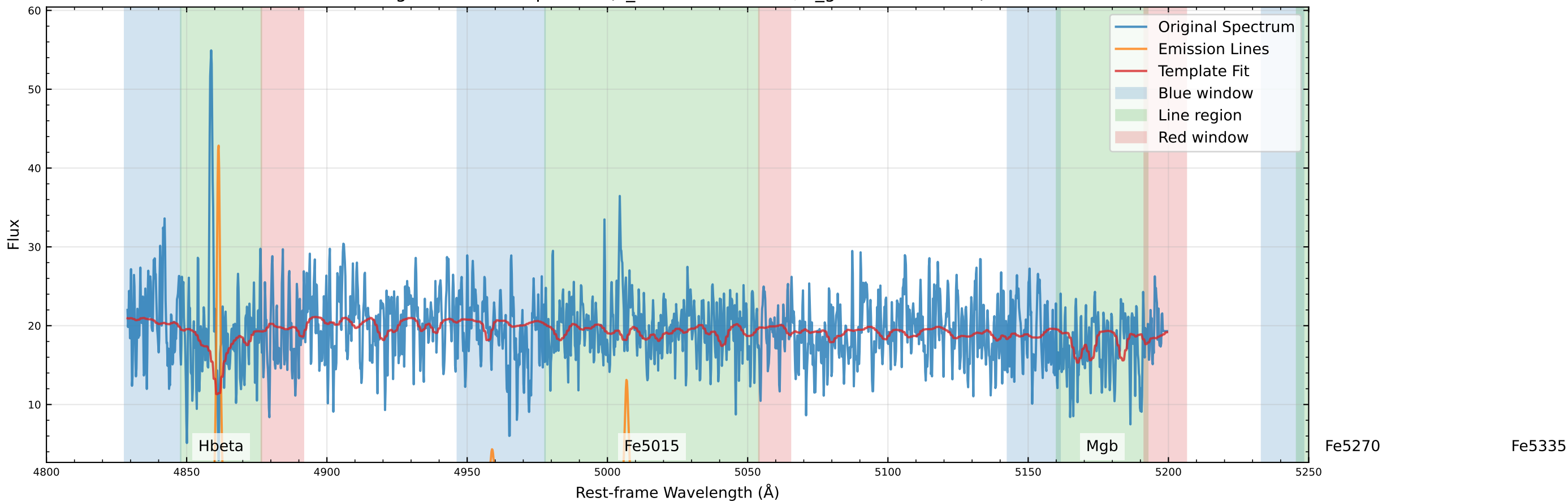
Original Data Comparison (v_star=-207.3 km/s, v_gas=-157.9 km/s)
