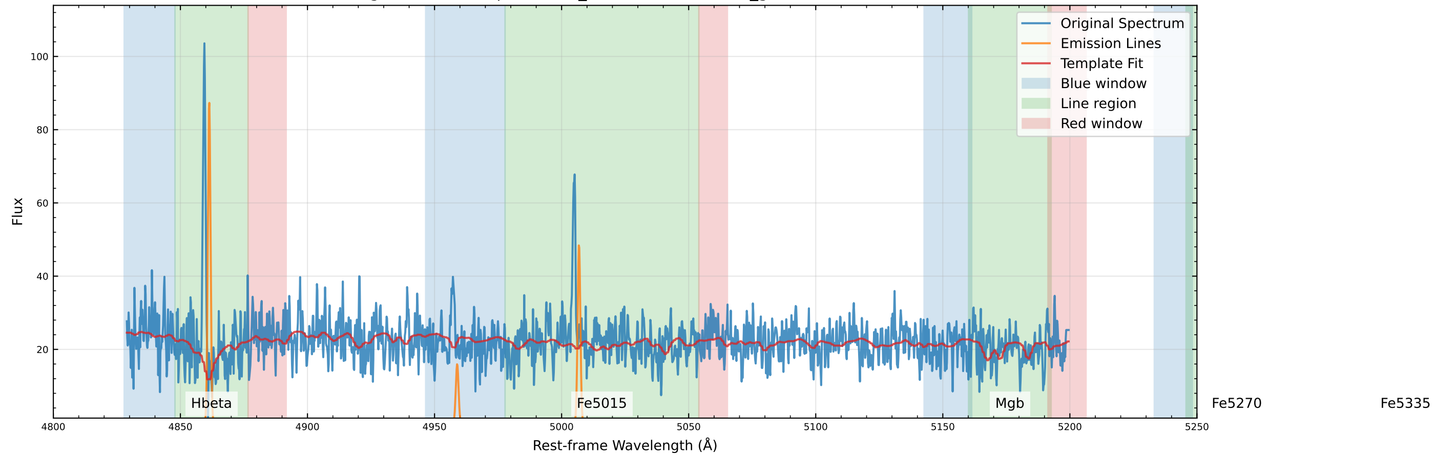
Original Data Comparison (v_star=-126.2 km/s, v_gas=-119.3 km/s)
