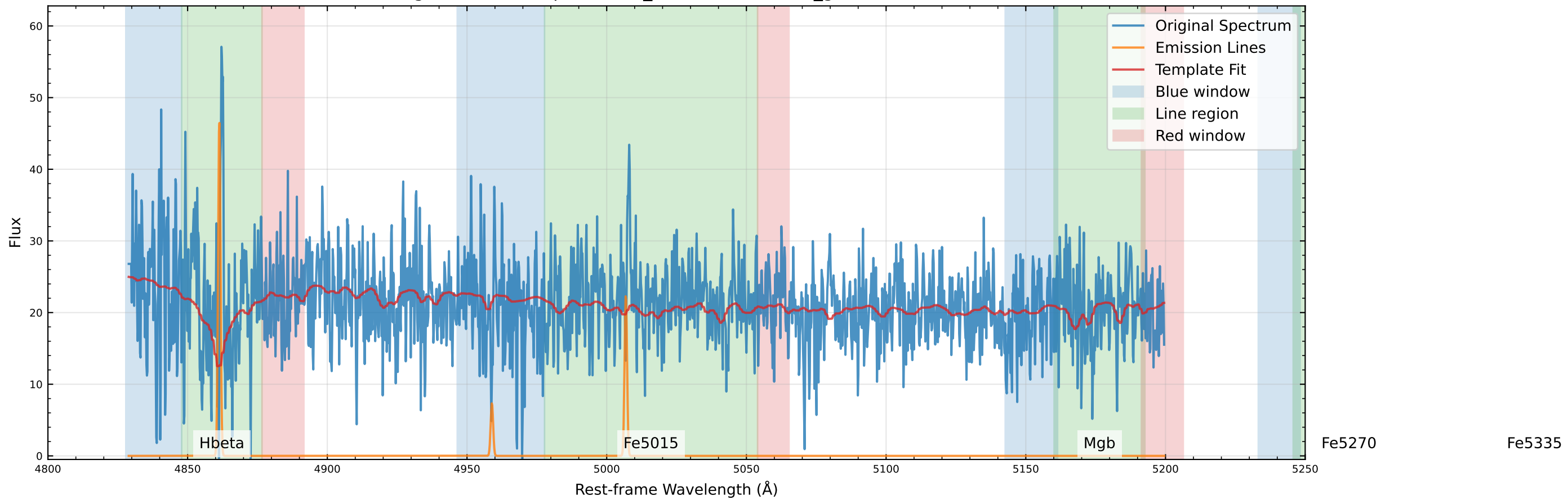
Original Data Comparison (v_star=63.6 km/s, v_gas=58.9 km/s)
