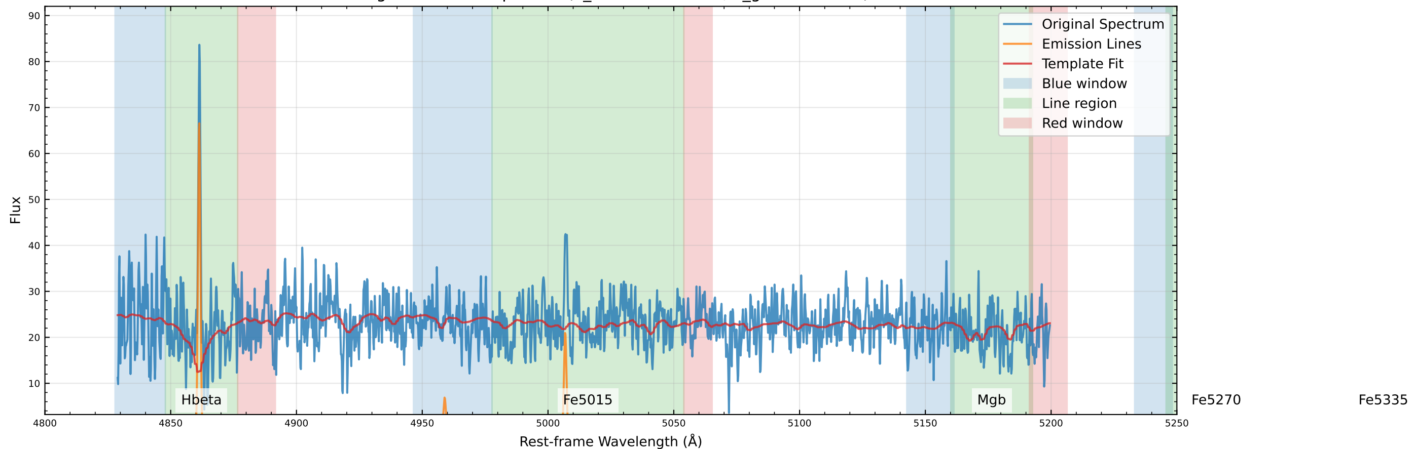
Original Data Comparison (v_star=-14.1 km/s, v_gas=5.0 km/s)
