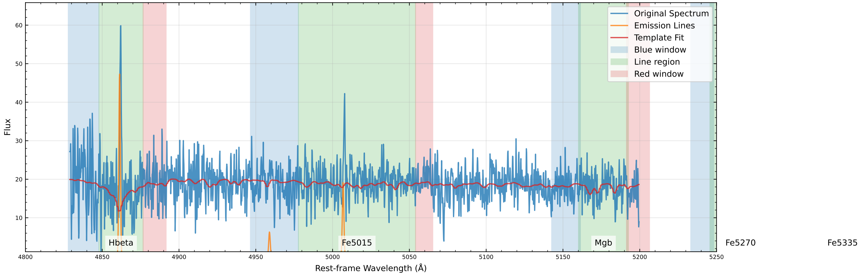
Original Data Comparison (v_star=49.7 km/s, v_gas=41.2 km/s)
