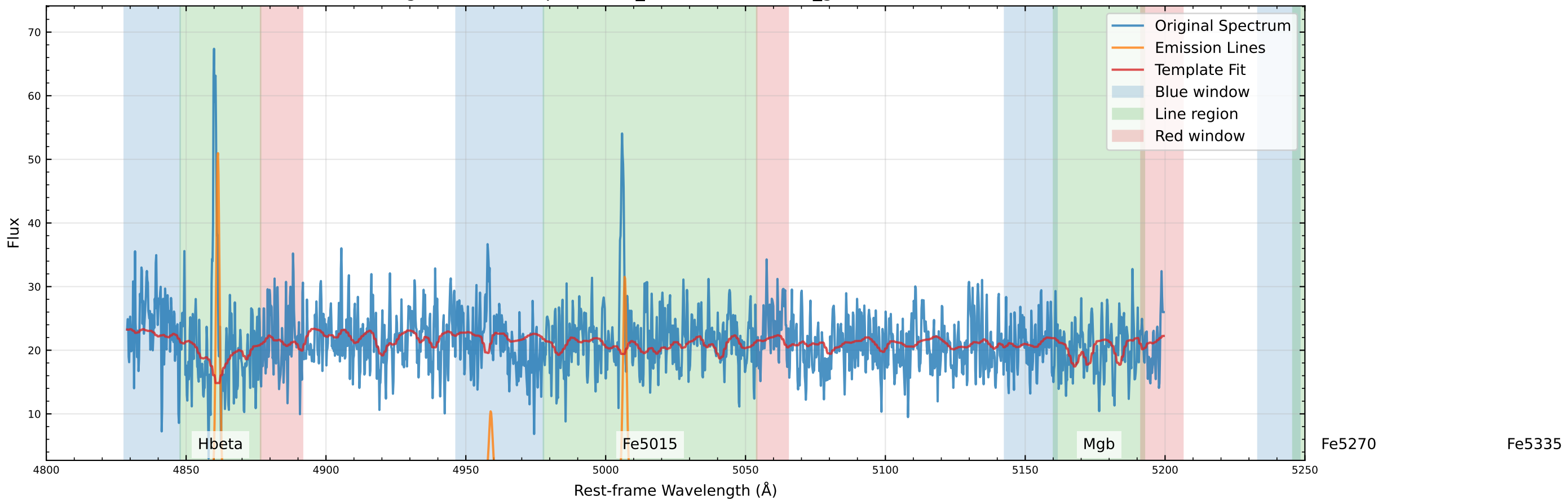
Original Data Comparison (v_star=-57.2 km/s, v_gas=-63.5 km/s)
