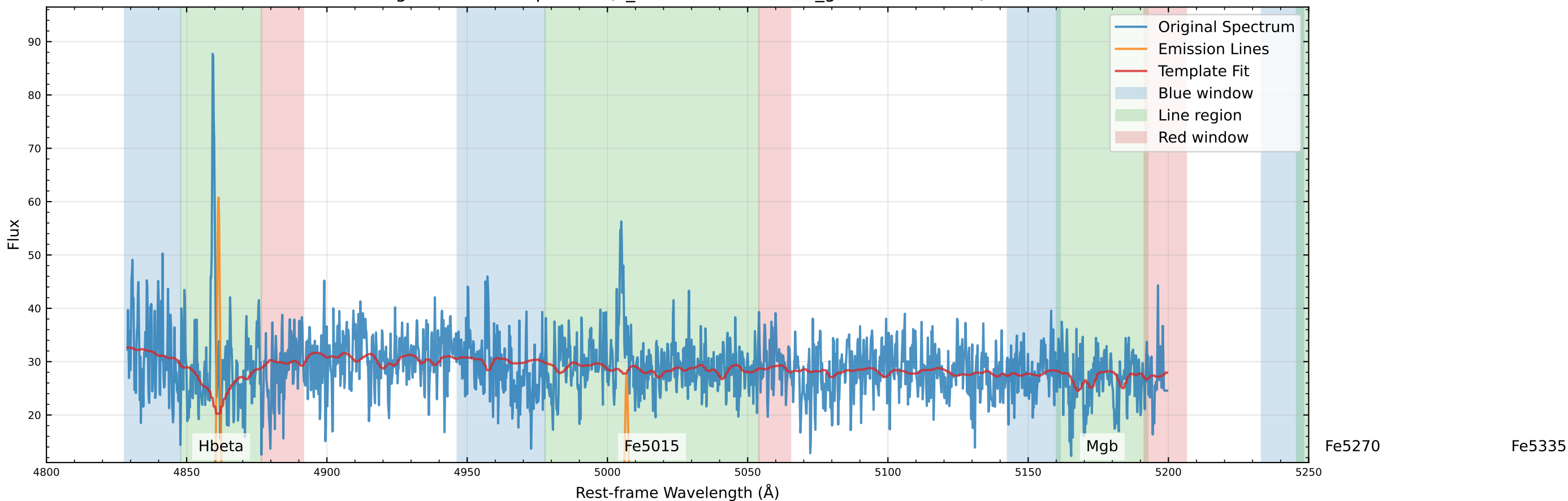
Original Data Comparison (v_star=-137.3 km/s, v_gas=-116.0 km/s)
