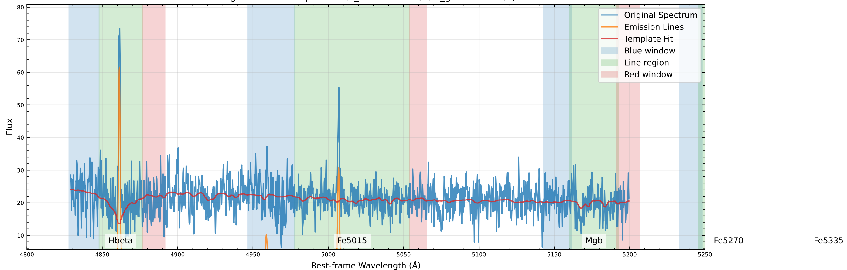
Original Data Comparison (v_star=4.7 km/s, v_gas=0.5 km/s)
