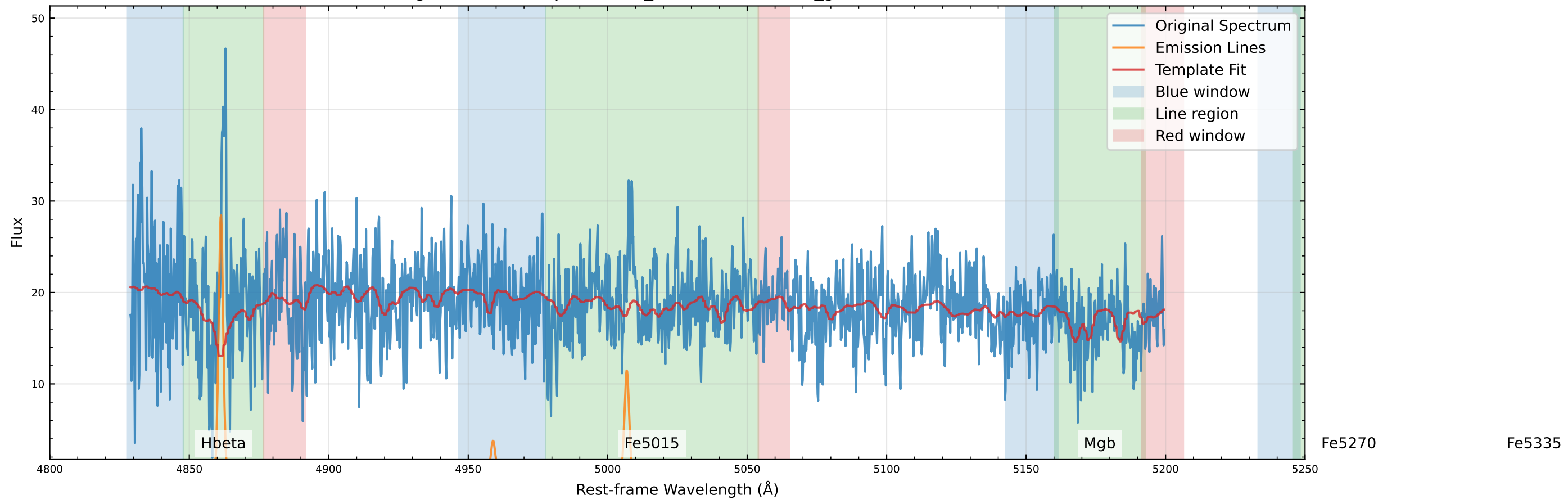
Original Data Comparison (v_star=58.5 km/s, v_gas=65.6 km/s)
