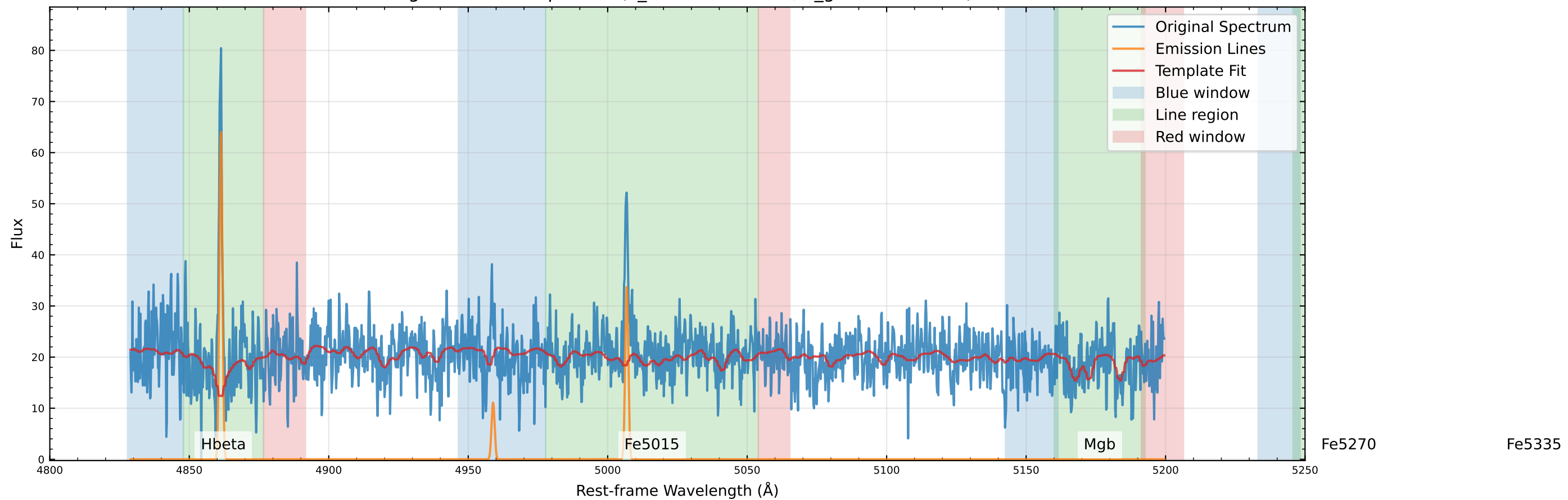
Original Data Comparison ( v_{\text{star}}=-24.3 km/s, v_{\text{gas}}=-10.1 km/s)
