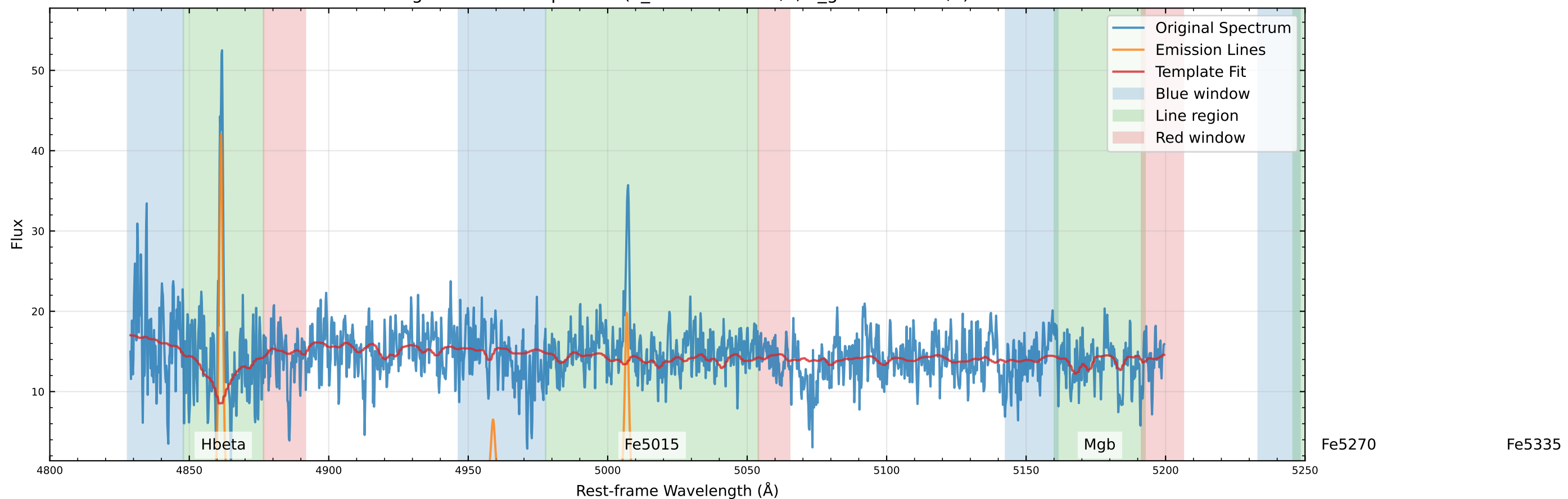
Original Data Comparison (v_star=-16.7 km/s, v_gas=10.2 km/s)
