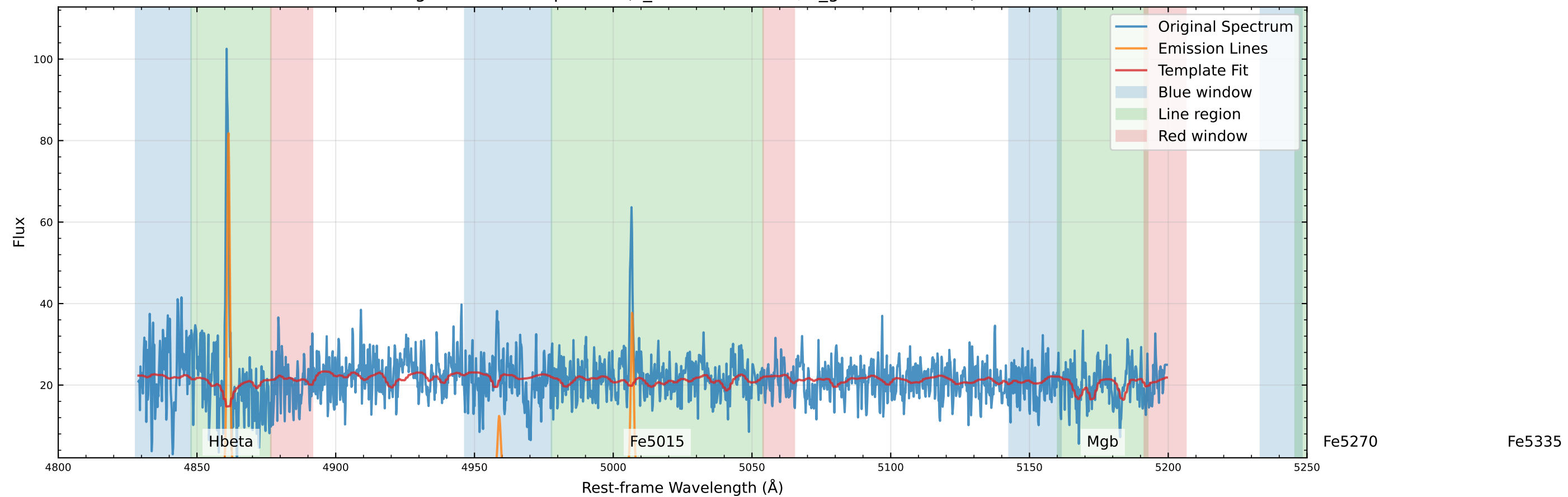
Original Data Comparison (v_star=-63.7 km/s, v_gas=-29.2 km/s)
