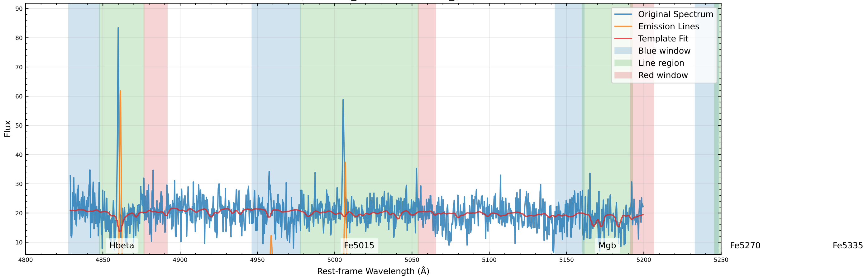
Original Data Comparison (v_star=-16.3 km/s, v_gas=-82.7 km/s)
