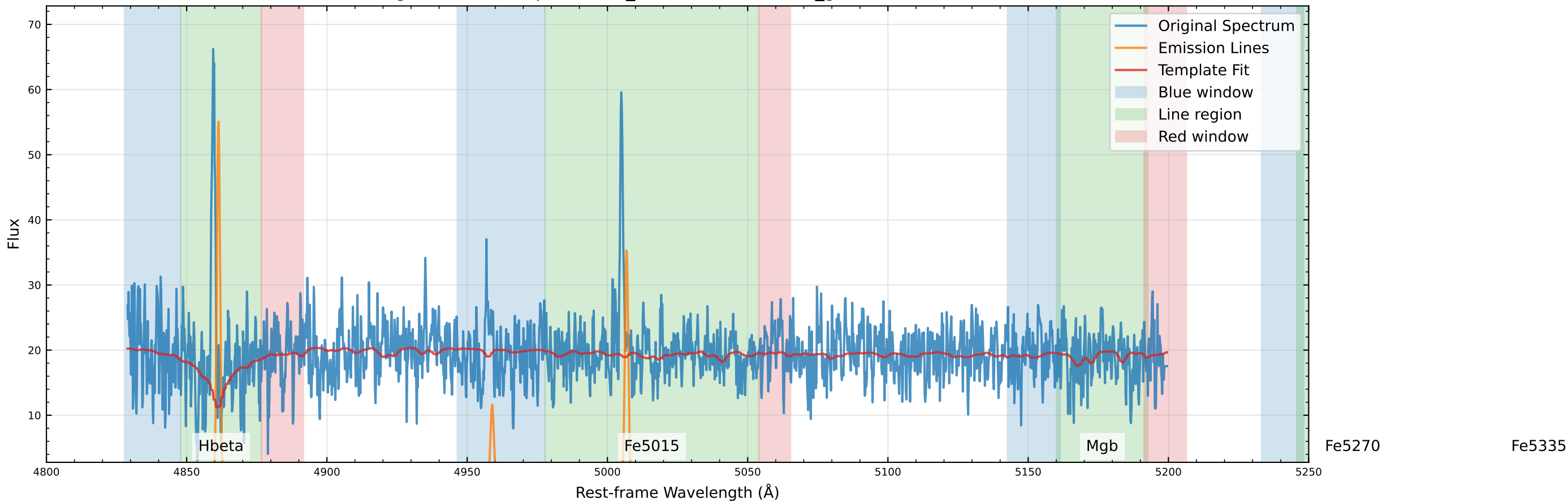
Original Data Comparison (v_star=-212.1 km/s, v_gas=-110.8 km/s)
