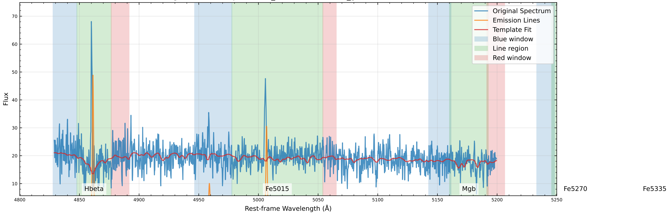
Original Data Comparison (v_star=-91.0 km/s, v_gas=-67.4 km/s)
