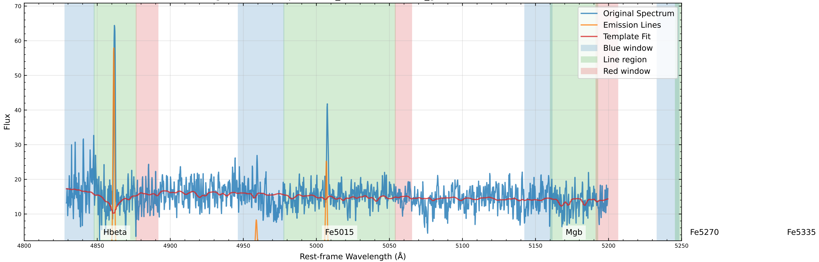
Original Data Comparison (v_star=50.6 km/s, v_gas=32.3 km/s)
