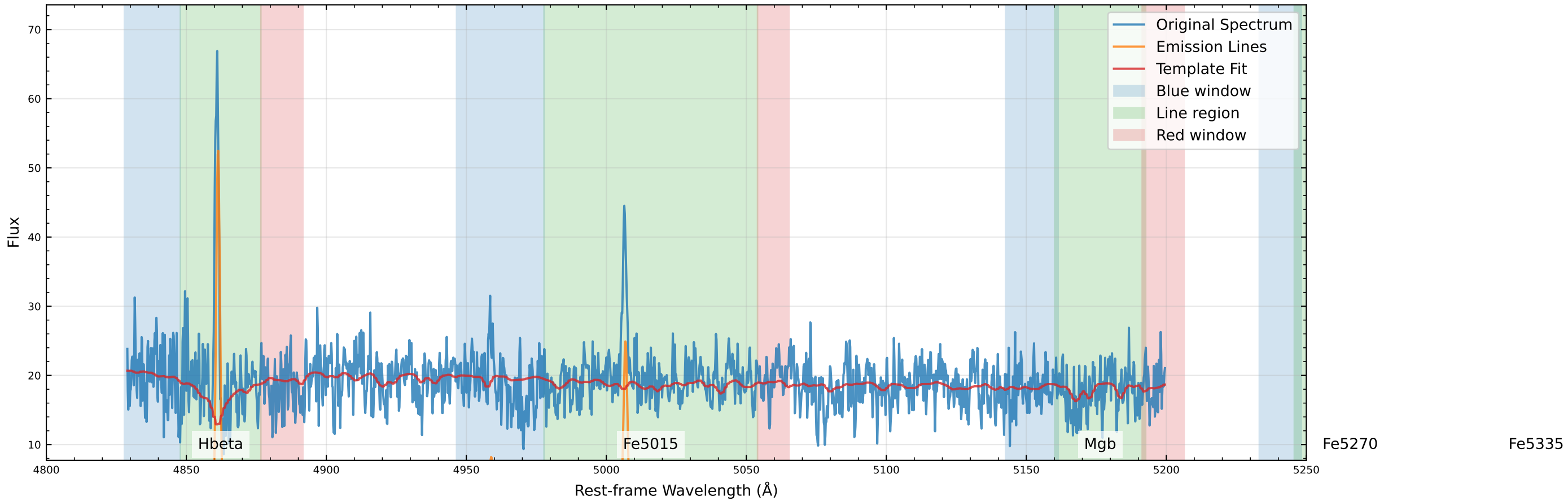
Original Data Comparison (v_star=-43.6 km/s, v_gas=-27.4 km/s)
