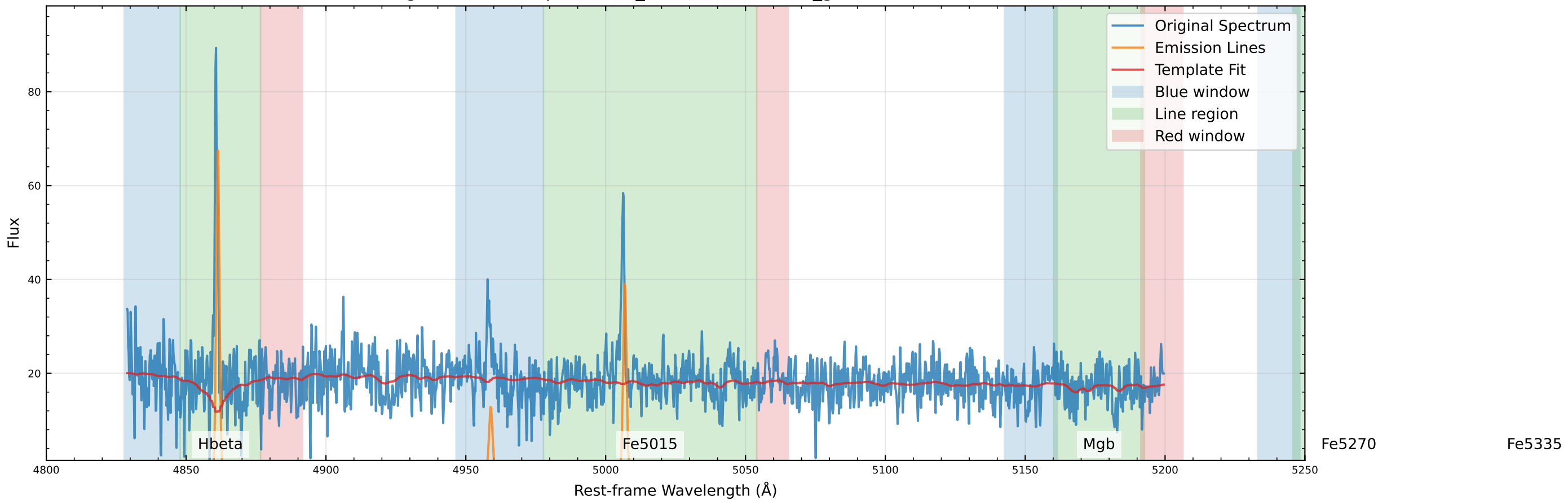
Original Data Comparison (v_star=-48.1 km/s, v_gas=-39.4 km/s)
