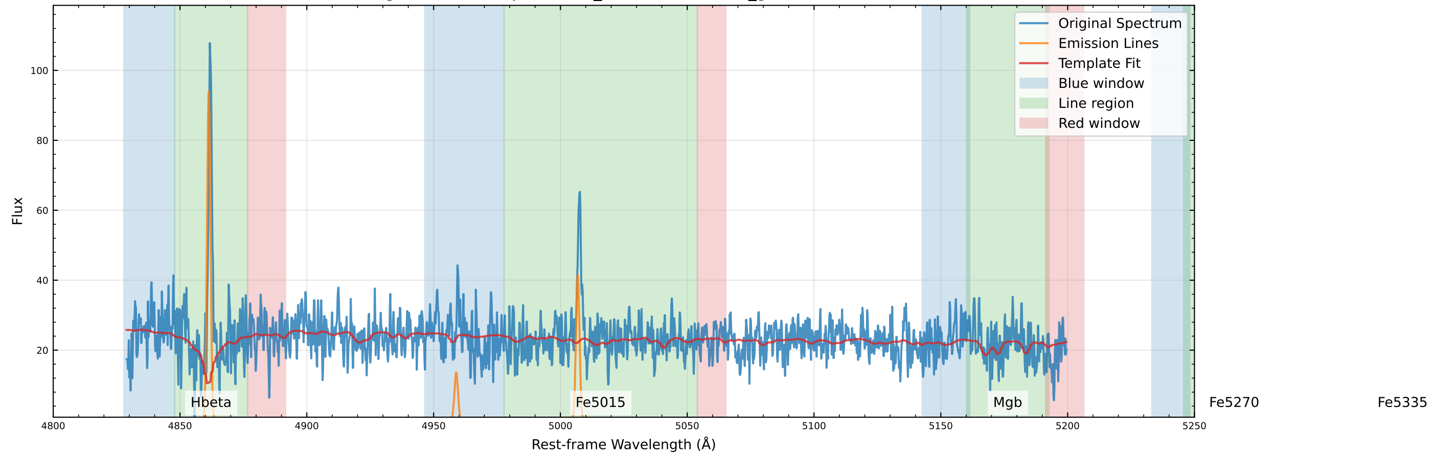
Original Data Comparison (v_star=32.2 km/s, v_gas=36.8 km/s)
