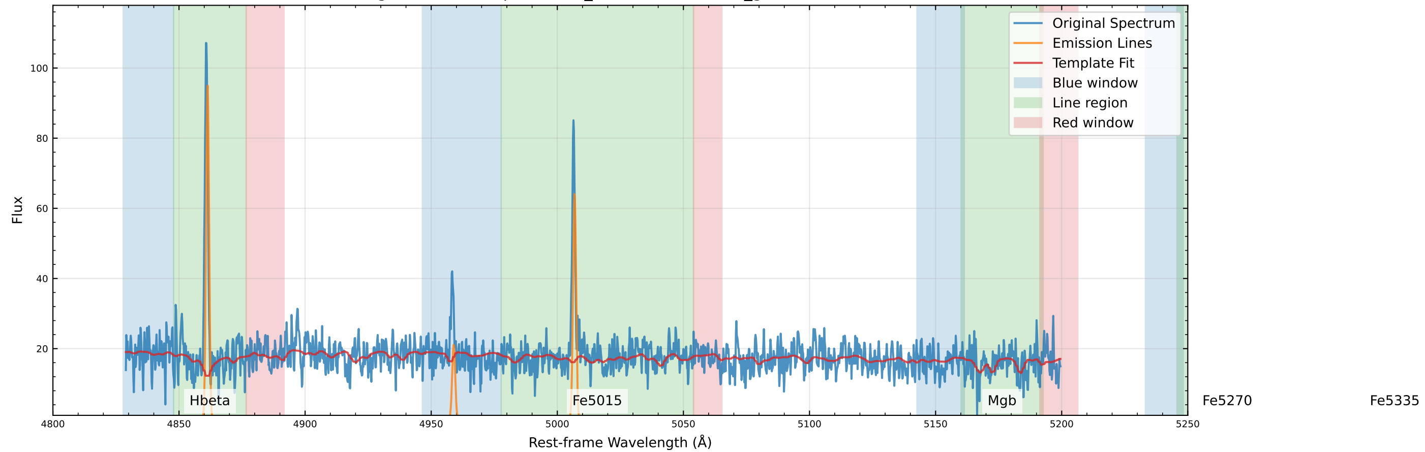
Original Data Comparison (v_star=-19.2 km/s, v_gas=-28.9 km/s)
