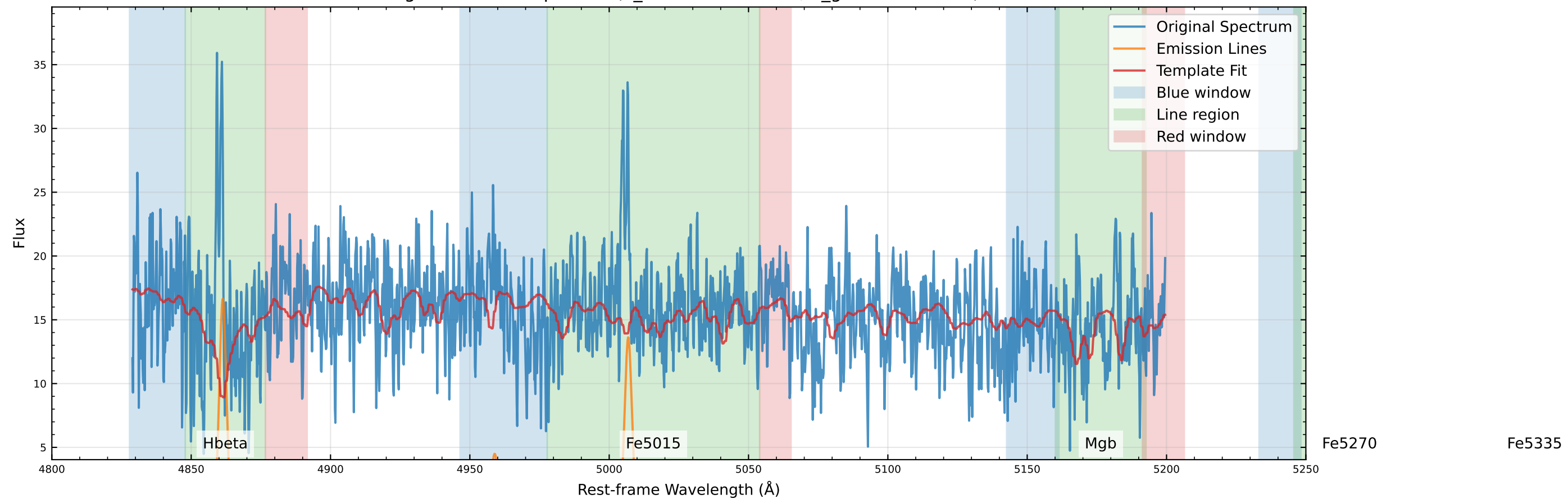
Original Data Comparison (v_star=-170.1 km/s, v_gas=-72.9 km/s)
