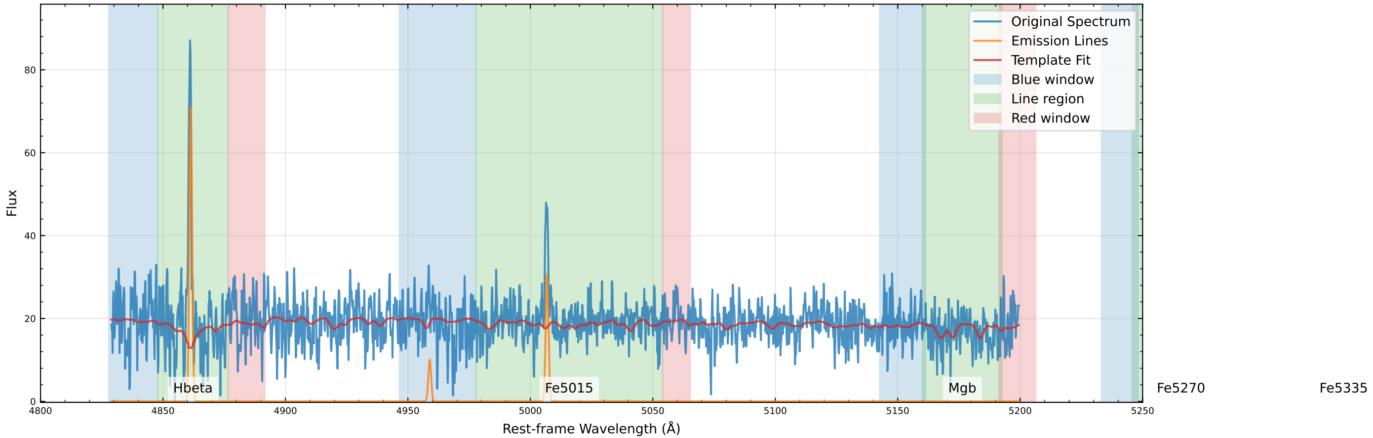
Original Data Comparison (v_star=-50.8 km/s, v_gas=-20.9 km/s)
