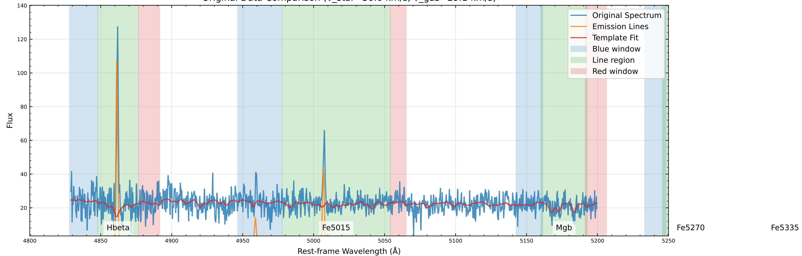
Original Data Comparison (v_star=30.0 km/s, v_gas=29.1 km/s)
