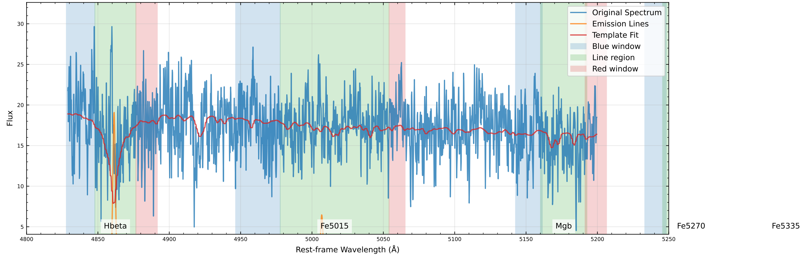
Original Data Comparison (v_star=-117.1 km/s, v_gas=-108.7 km/s)
