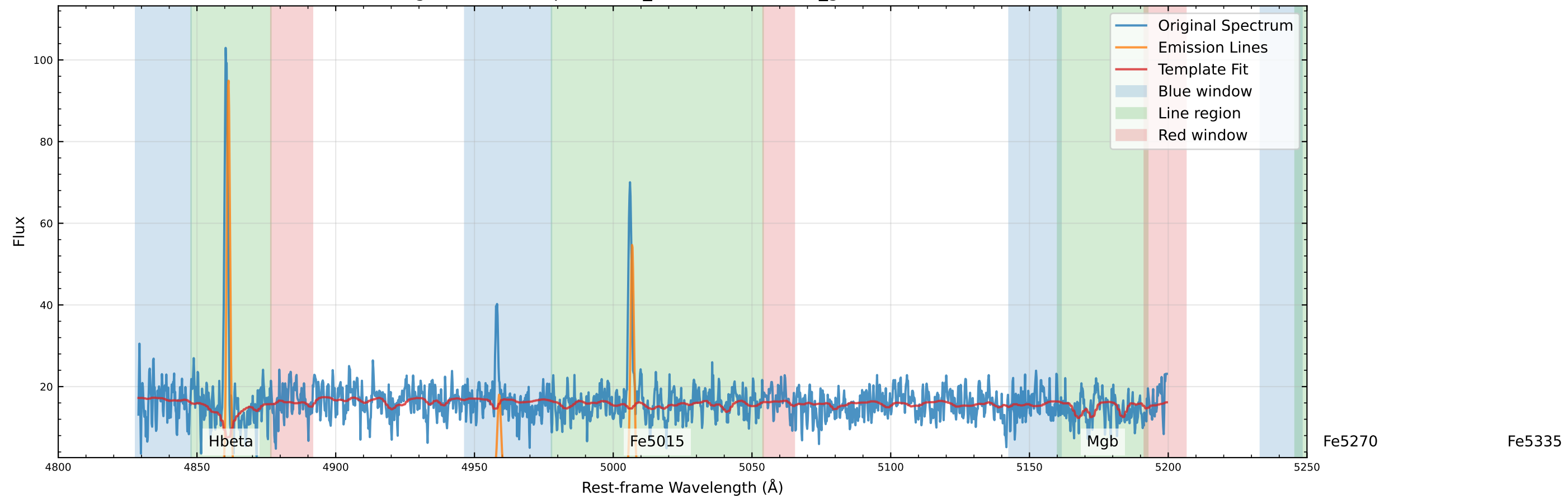
Original Data Comparison (v_star=-65.0 km/s, v_gas=-50.4 km/s)
