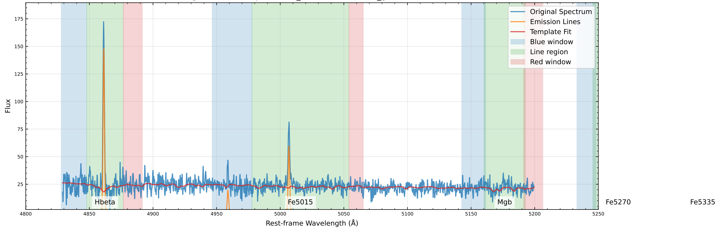
Original Data Comparison (v_star=-34.1 km/s, v_gas=-5.8 km/s)
