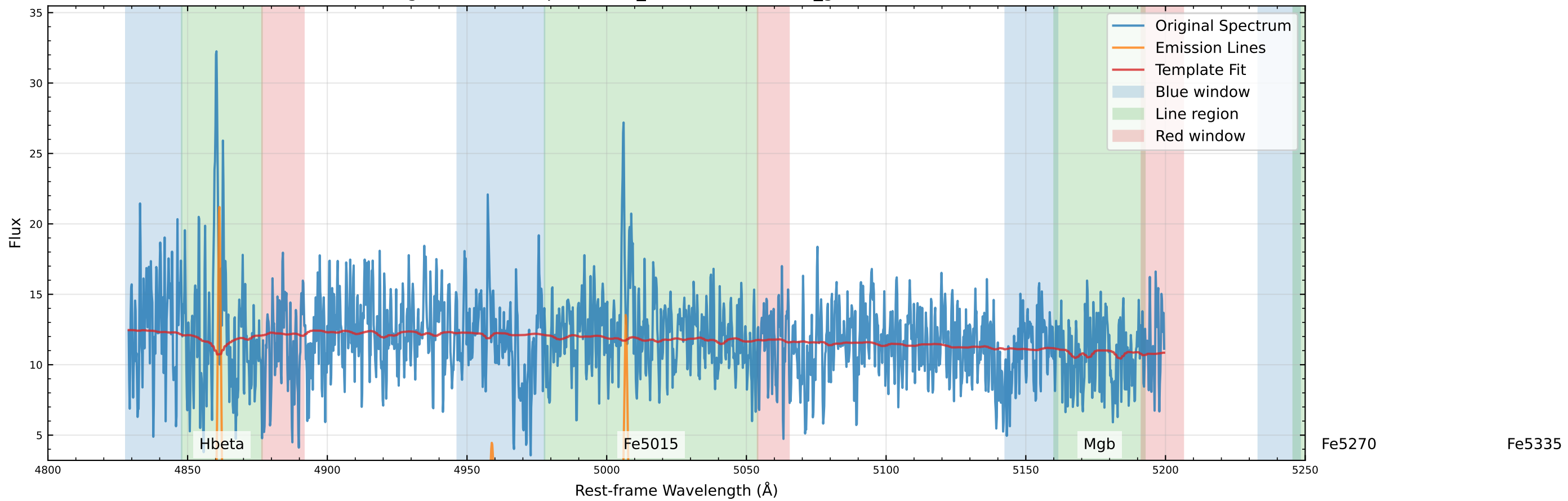
Original Data Comparison (v_star=-12.3 km/s, v_gas=-66.0 km/s)
