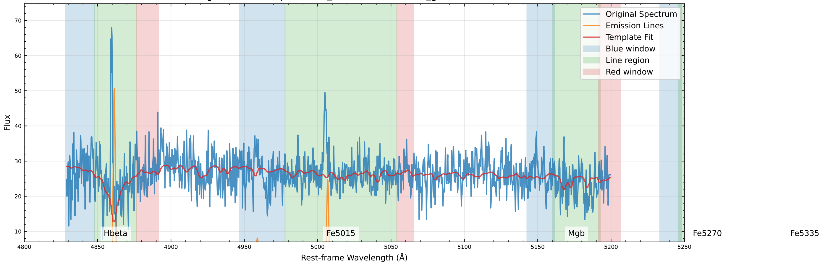
Original Data Comparison (v_star=-116.6 km/s, v_gas=-111.8 km/s)
