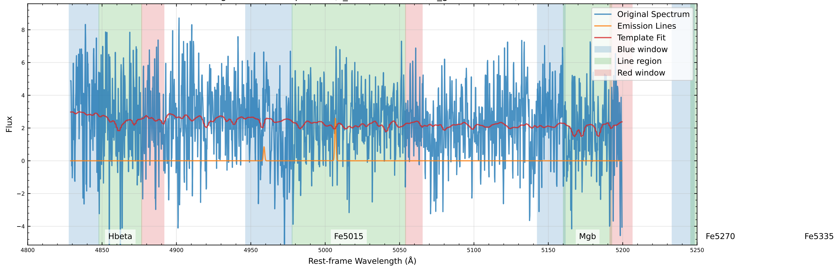
Original Data Comparison (v_star=-26.5 km/s, v_gas=17.5 km/s)
