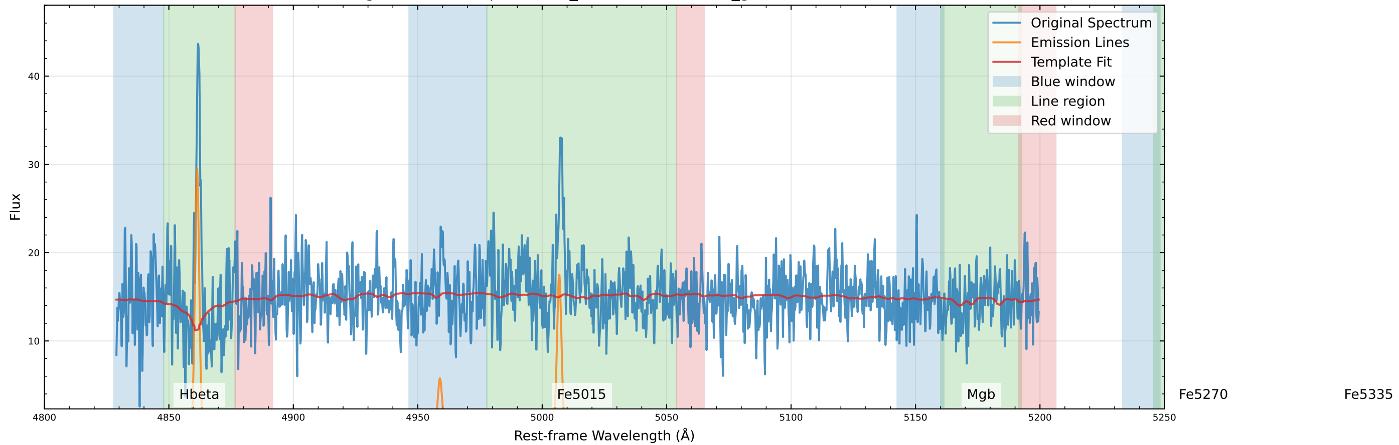
Original Data Comparison ( v_{\text{star}}=150.0 km/s, v_{\text{gas}}=32.4 km/s)
