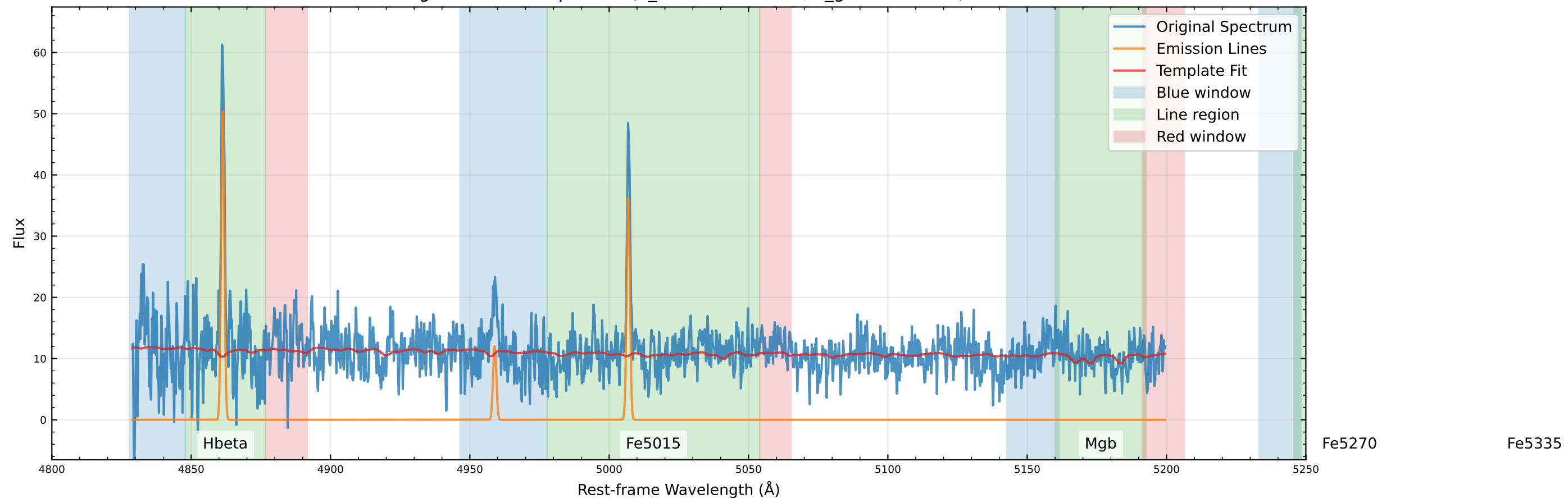
Original Data Comparison (v_star=-31.1 km/s, v_gas=2.2 km/s)
