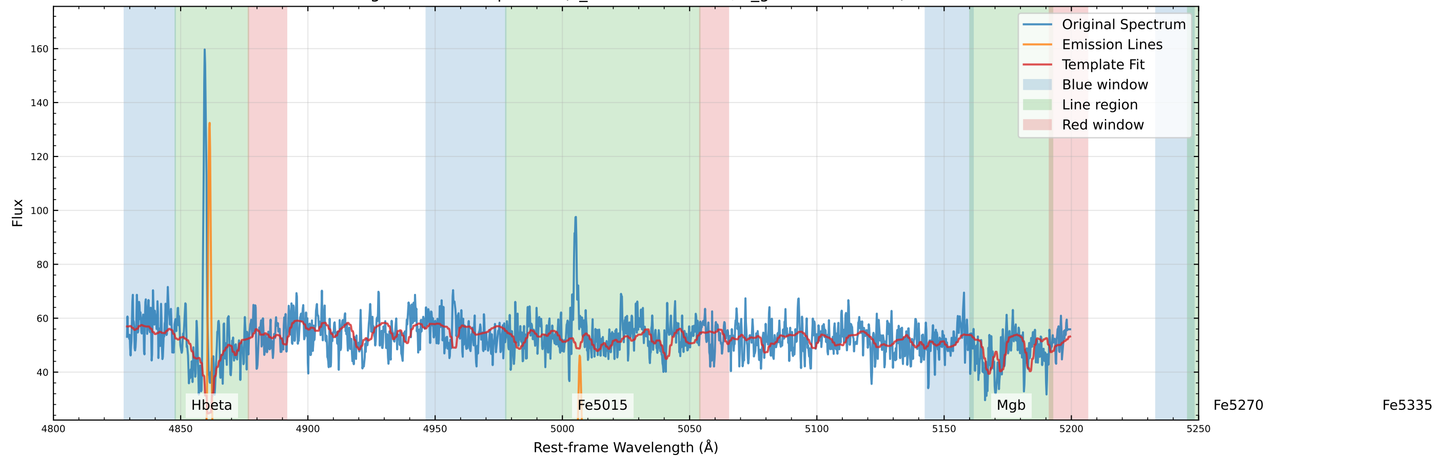
Original Data Comparison (v_star=-113.4 km/s, v_gas=-108.6 km/s)
