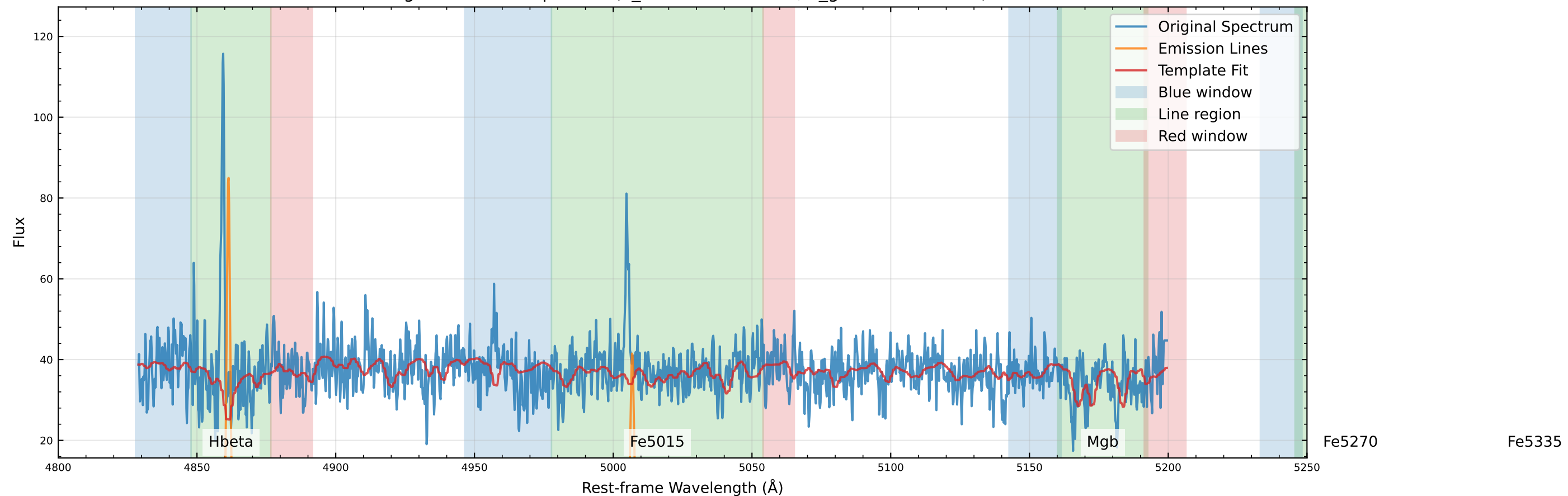
Original Data Comparison (v_star=-119.7 km/s, v_gas=-124.9 km/s)
