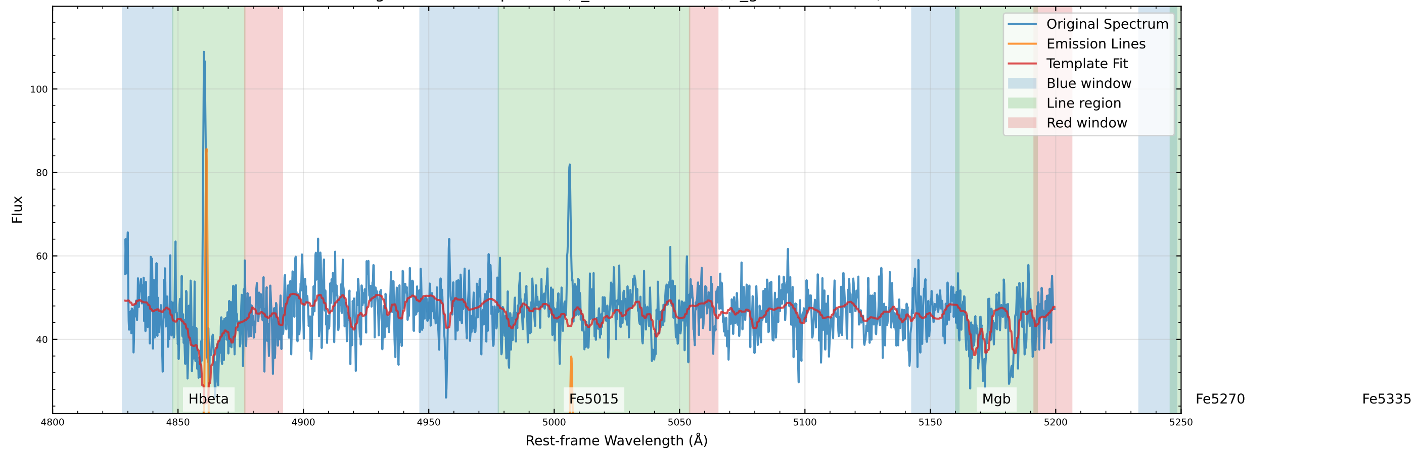
Original Data Comparison (v_star=-62.1 km/s, v_gas=-50.1 km/s)
