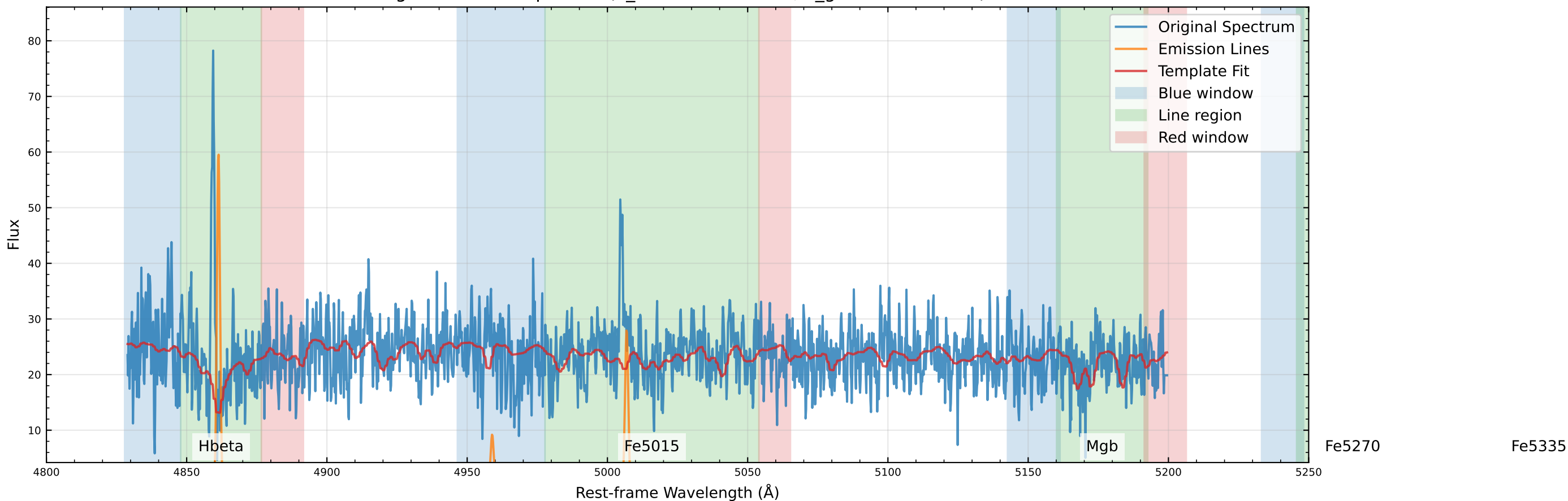
Original Data Comparison (v_star=-114.6 km/s, v_gas=-119.4 km/s)
