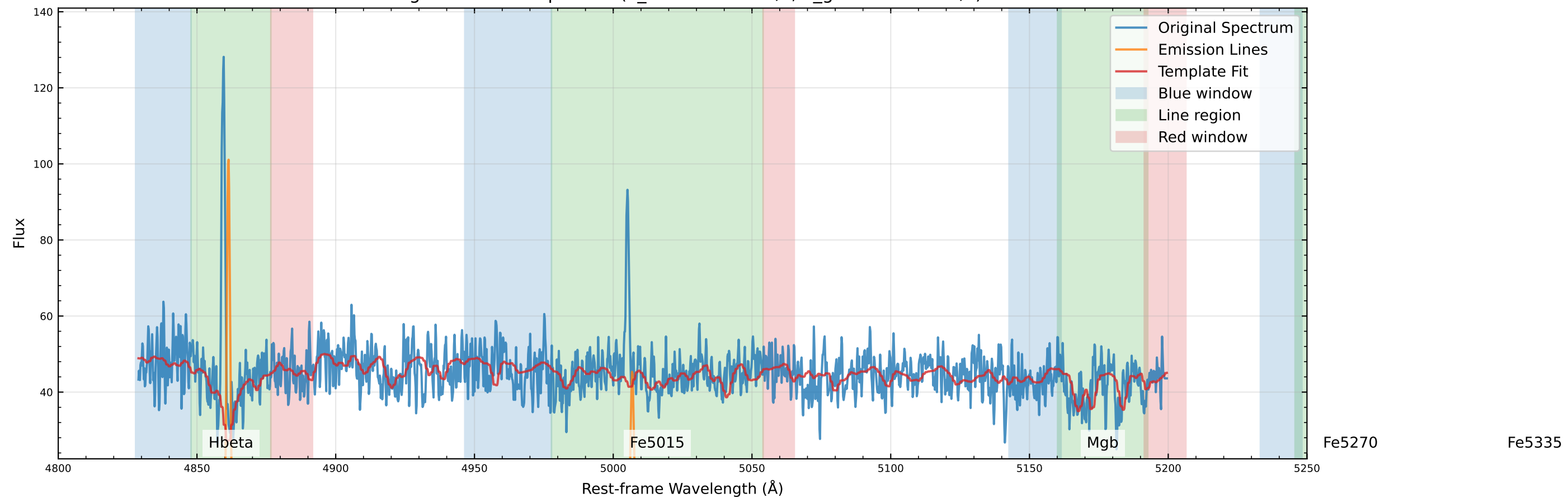
Original Data Comparison (v_star=-98.7 km/s, v_gas=-111.8 km/s)
