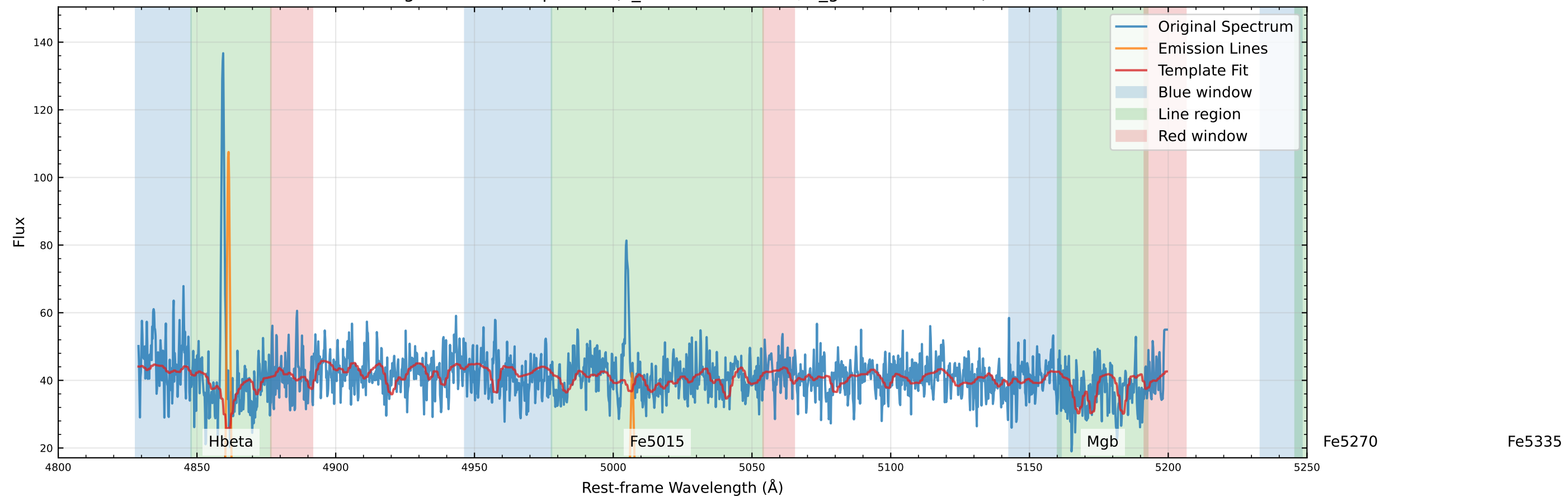
Original Data Comparison (v_star=-107.9 km/s, v_gas=-121.6 km/s)
