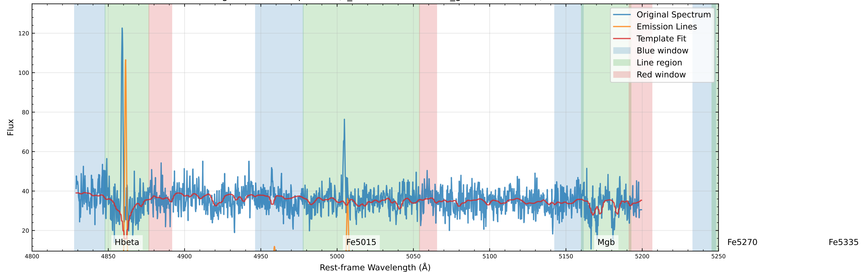
Original Data Comparison (v_star=-130.6 km/s, v_gas=-137.8 km/s)
