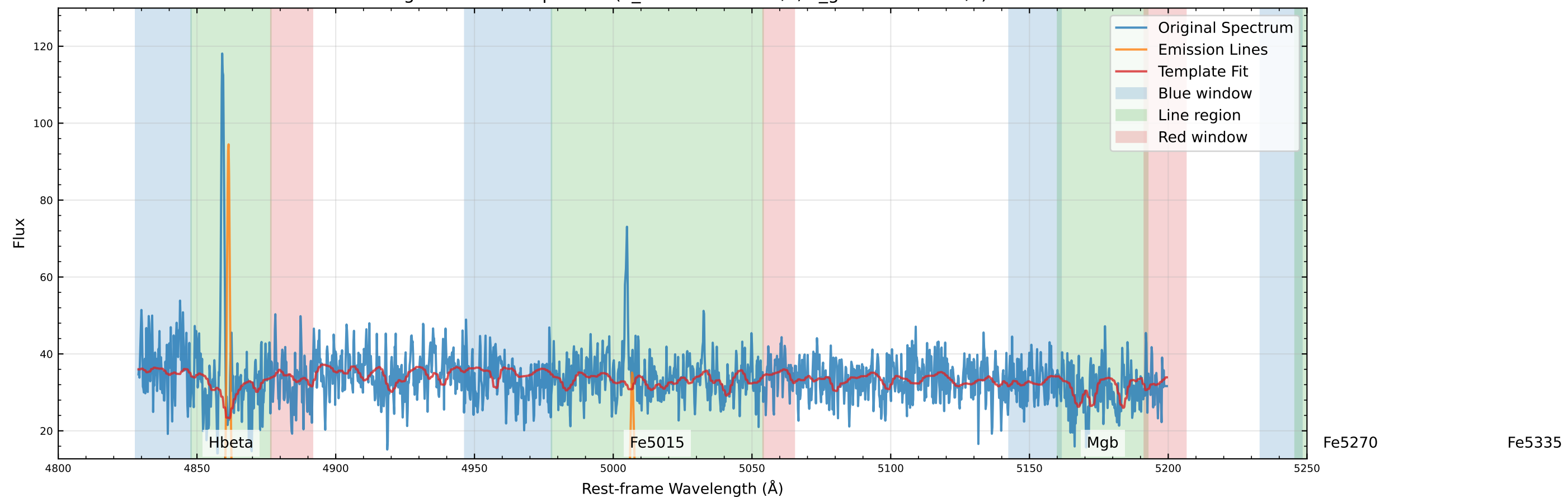
Original Data Comparison (v_star=-108.3 km/s, v_gas=-128.5 km/s)
