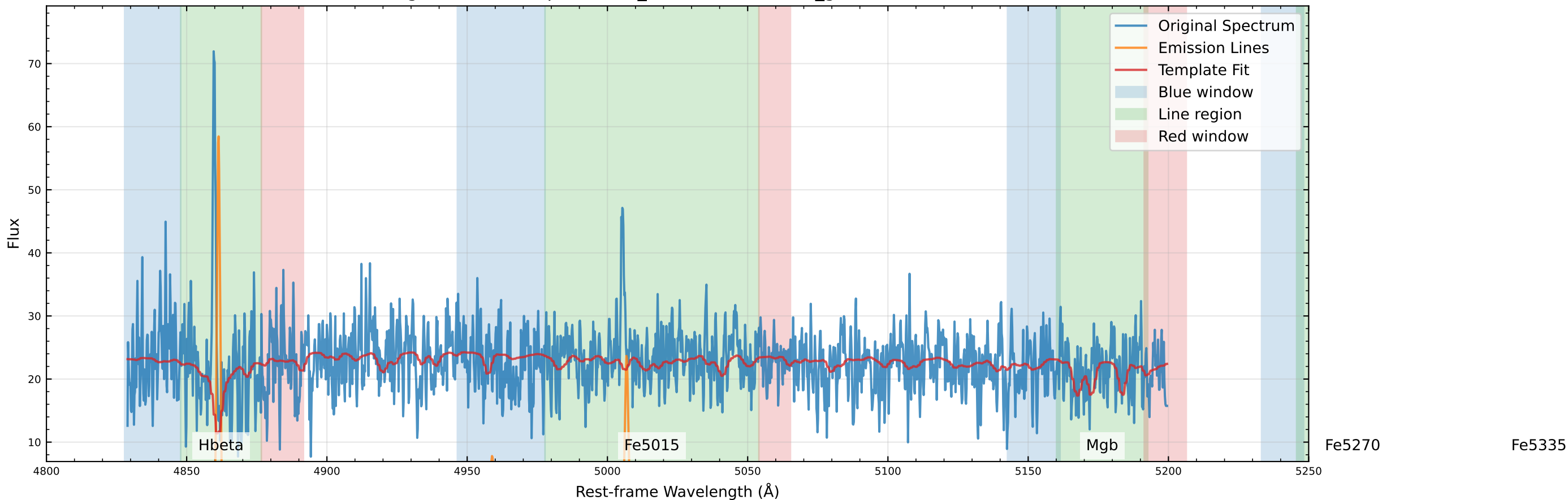
Original Data Comparison (v_star=-61.5 km/s, v_gas=-92.3 km/s)
