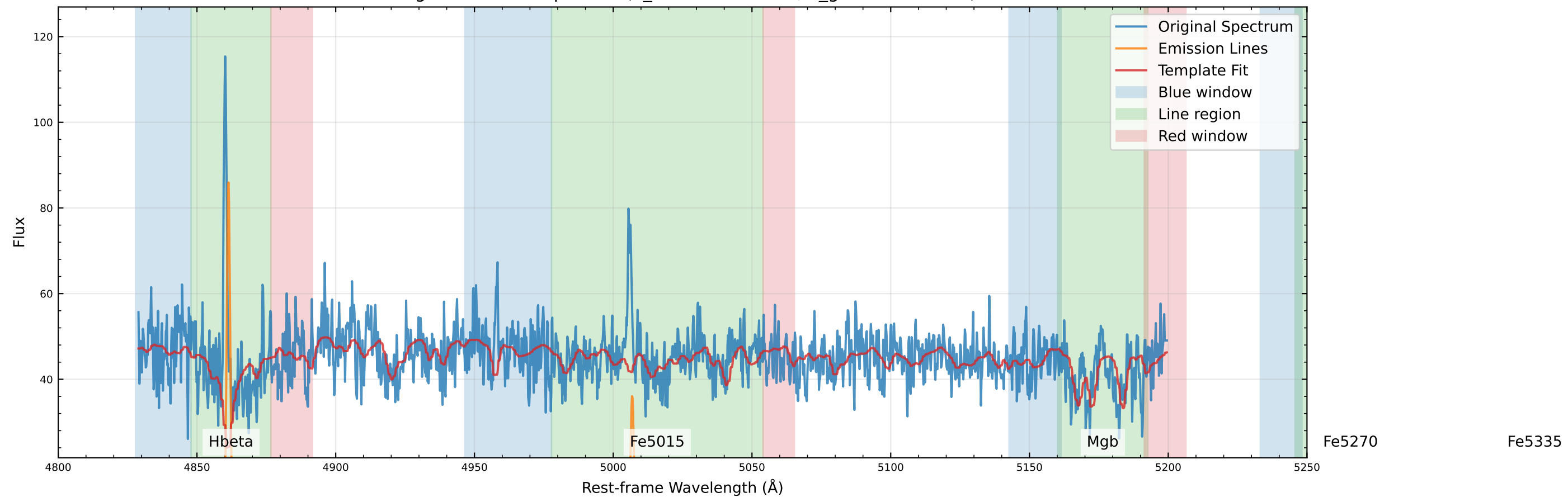
Original Data Comparison (v_star=-90.9 km/s, v_gas=-69.6 km/s)
