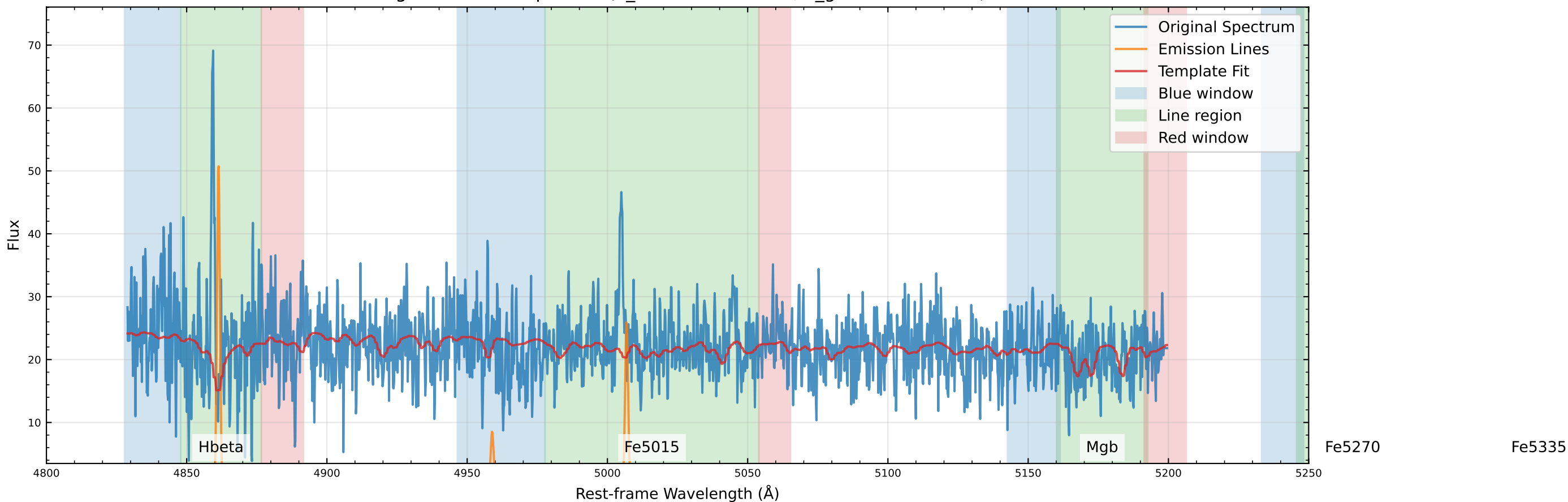
Original Data Comparison (v_star=-113.4 km/s, v_gas=-123.3 km/s)
