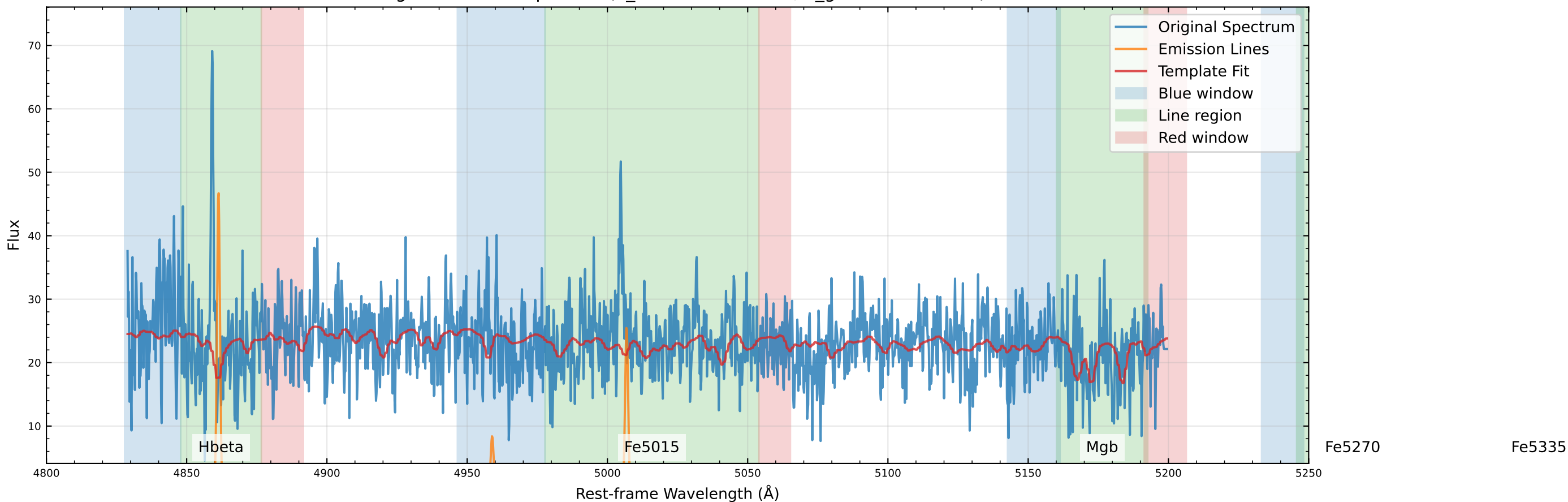
Original Data Comparison (v_star=-129.1 km/s, v_gas=-135.3 km/s)
