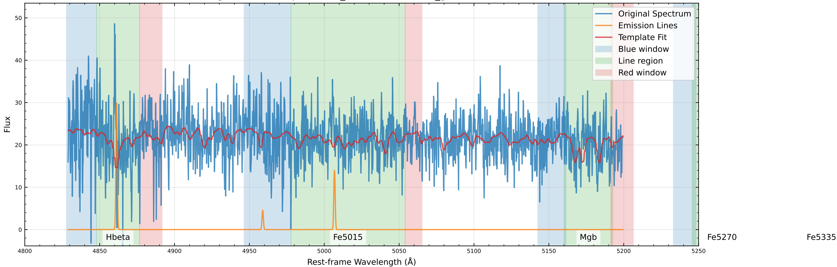
Original Data Comparison (v_star=-66.4 km/s, v_gas=-70.9 km/s)
